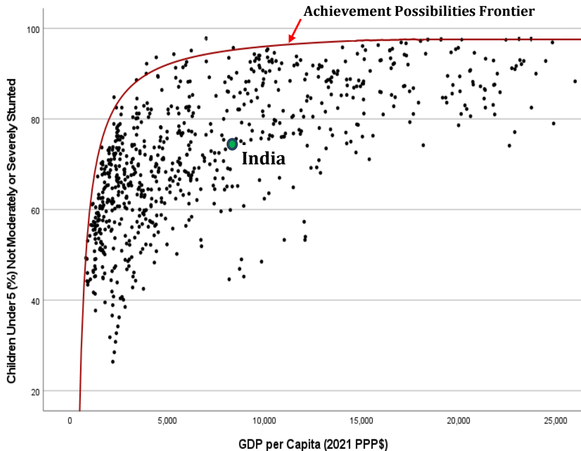
Figure 1: Achievement Possibilities Frontier for “Percentage of Children Not Stunted”
