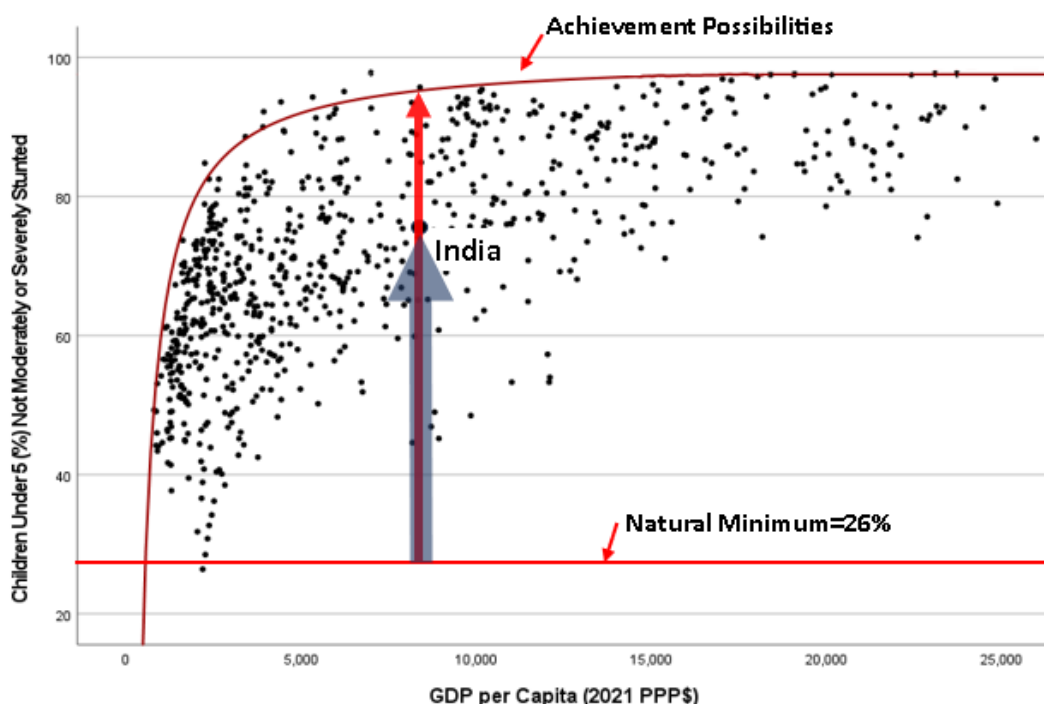
Figure 2: Rescaling the indicator scores
