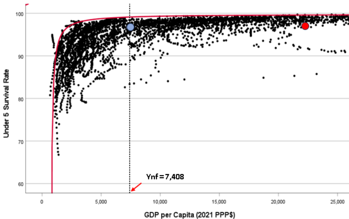
Figure 4: Example Achievement possibilities frontier (APF) with asymptotic peak
